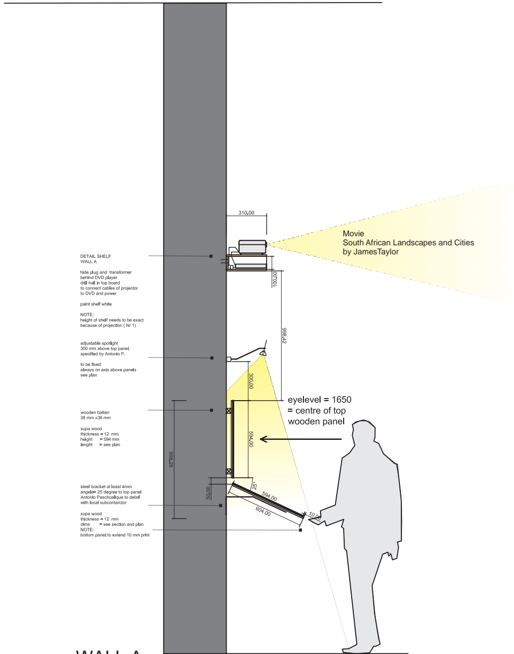
WALL A TYPICAL SECTION
